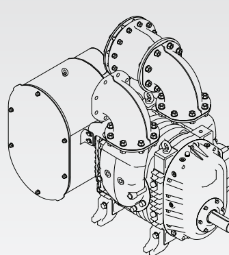
Fig.3 Positive displacement vacuum pump
